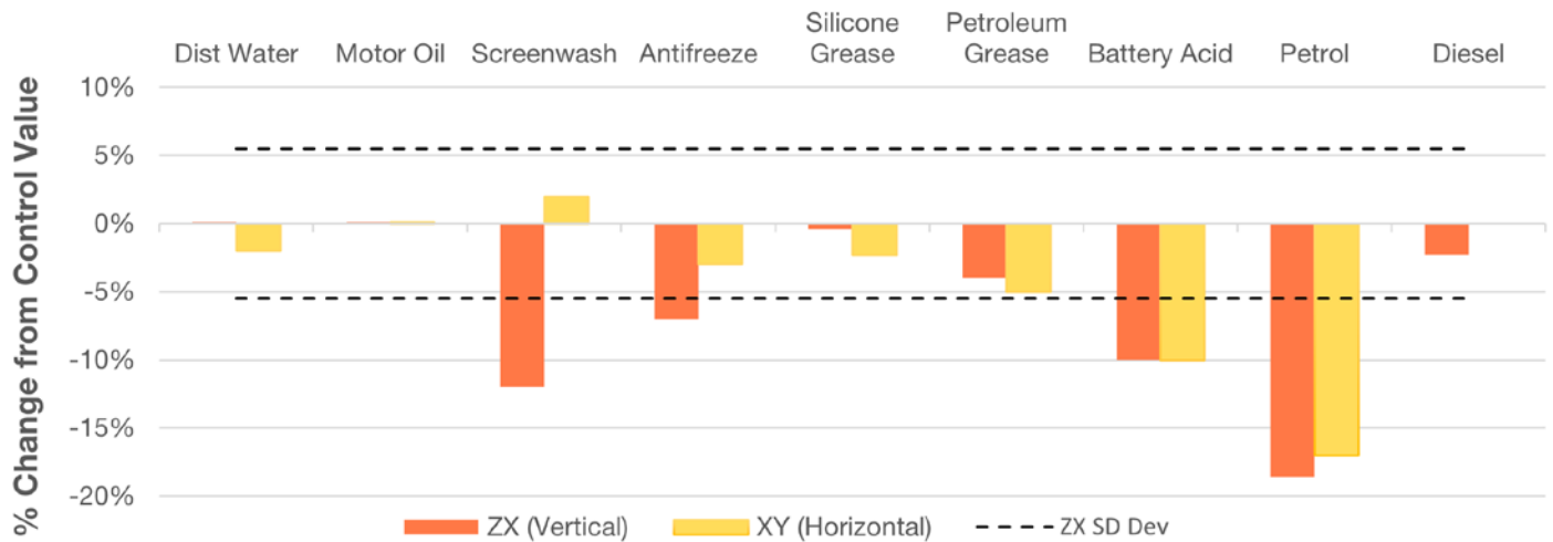
PA12 Youngs Modulus % Change from Nominal
