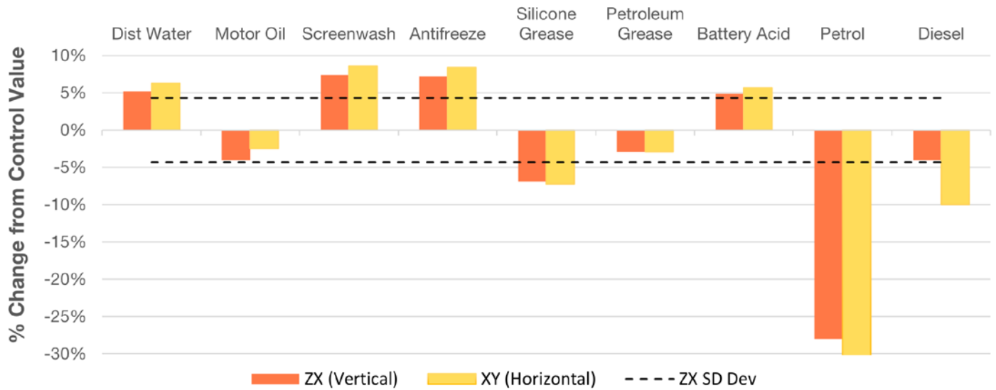
PP UTS % Change from Nominal
