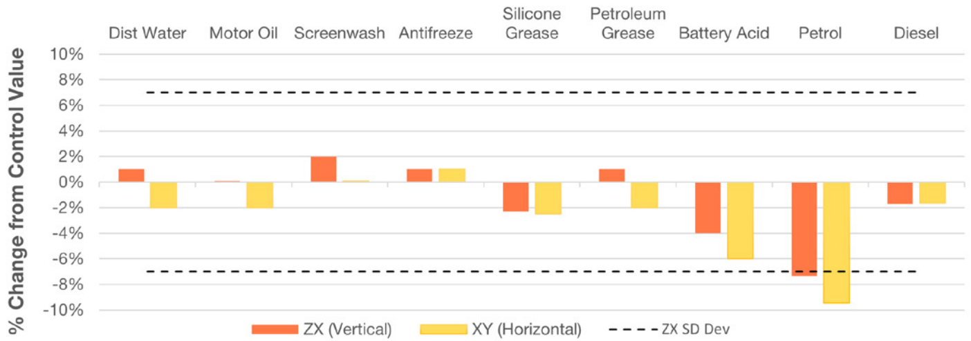
PA12 UTS % Change from Nominal
