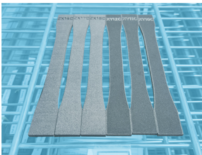
Figure 2. Tensile control specimens (marked C with matching pair number) on preconditioning racks.
